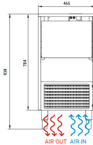
FRONTAL VIEW
